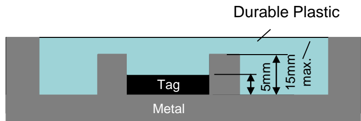
Cross Section of Manhole Lid
